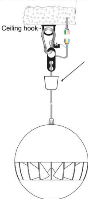
After finish installation, close the cable connection with the cover provided
